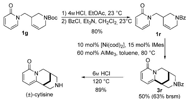
Scheme 2. Application of the endo -cyclization mode for the synthesis of the lupin alkaloid (±)-cytosine. brsm = based on recovered starting material, Bz = benzoyl.
